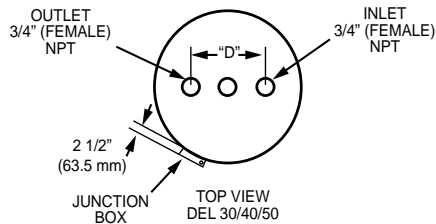
TOP VIEW DEL 30/40/50
