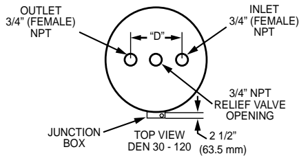
TOP VIEW DEN 30-120
