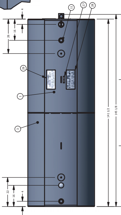
DETAIL B
