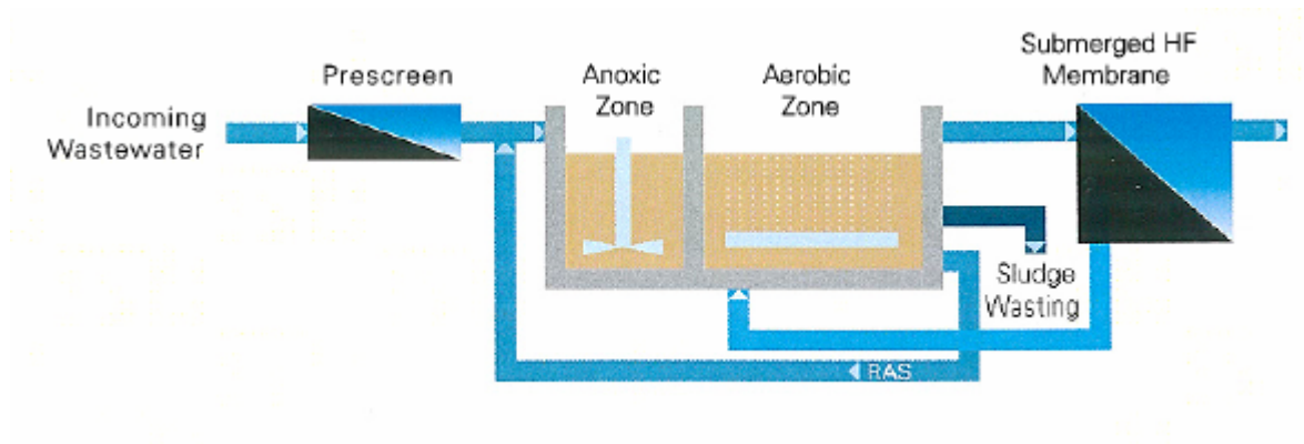
Figure 2. Immersed MBR configuration, including nitrogen removal steps.
