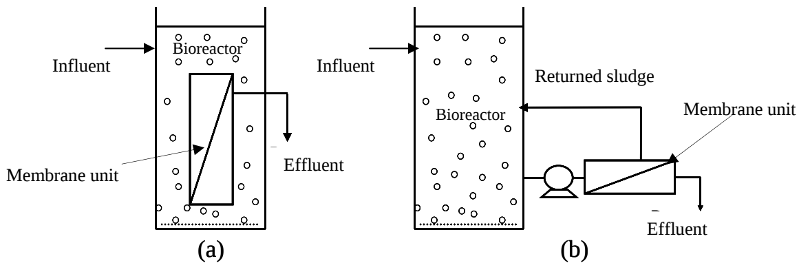
Figure 1. Two MBR configurations: (a) immersed (Im) and (b) Sidestream (SS).
