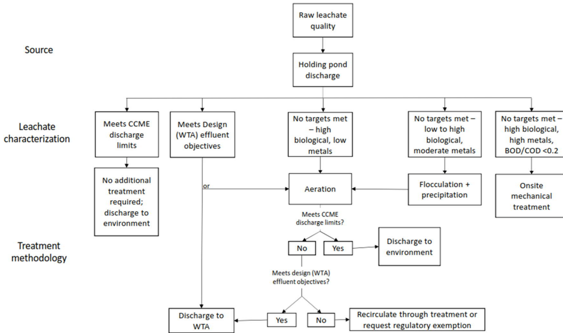
Figure 1. Recommended treatment considerations based on leachate characterization. Note that recommended management approaches will change based on actual leachate quality and quantity. Should any mechanical system need to be installed, power to the site will need to be considered.
