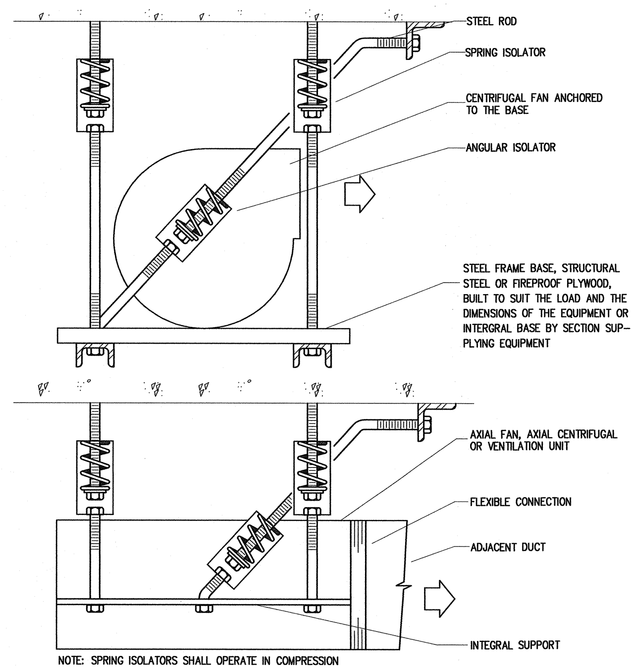
4 SUSPENDED EQUIPMENT (TYPE VI) M2 NTS
