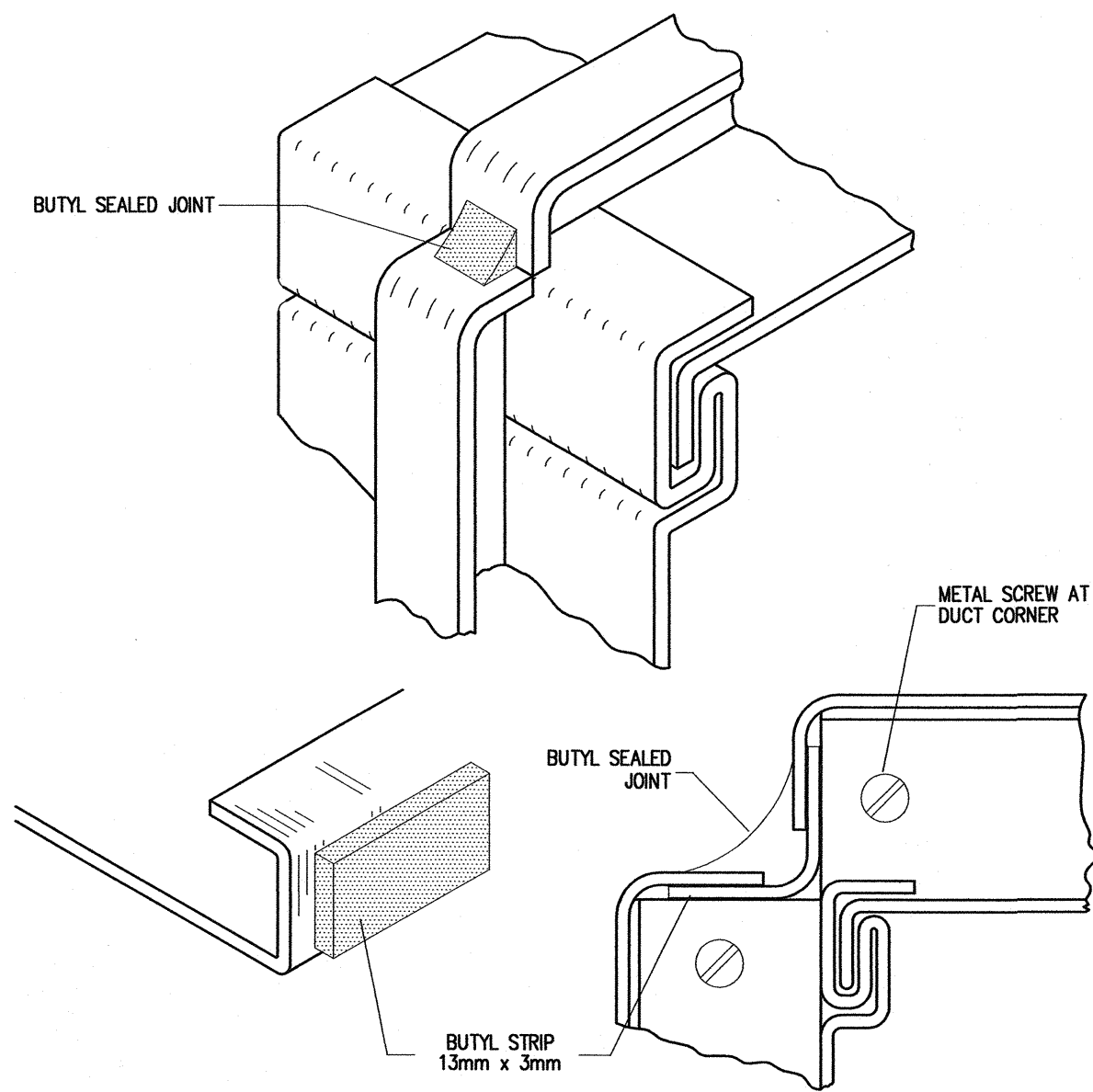
1 SEALED JOINT FOR LOW PRESSURE RECTANGULAR DUCT M2 NTS
