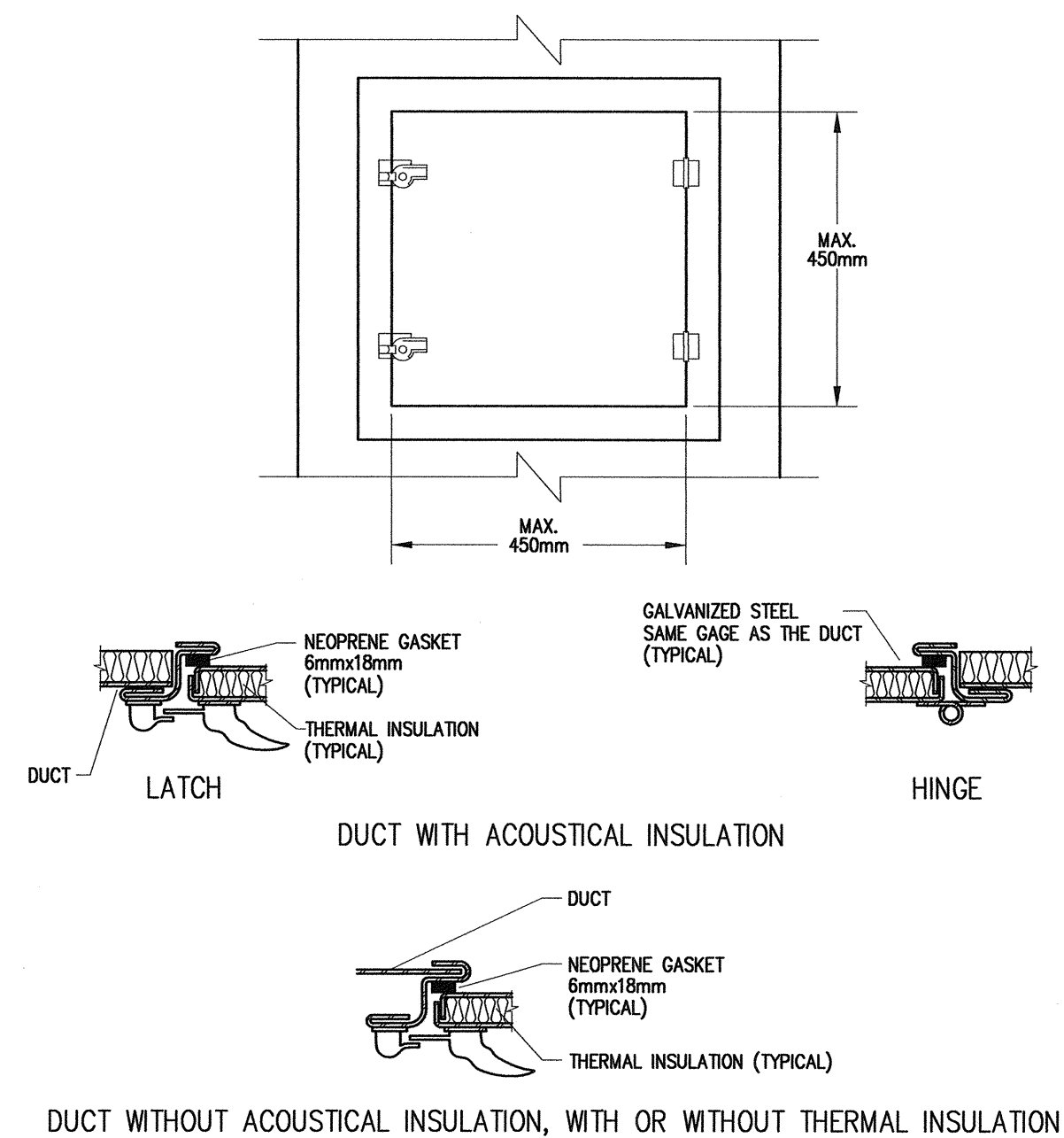
5 ACCESS DOOR FOR LOW PRESSURE RECTANGULAR DUCT M2 NTS
