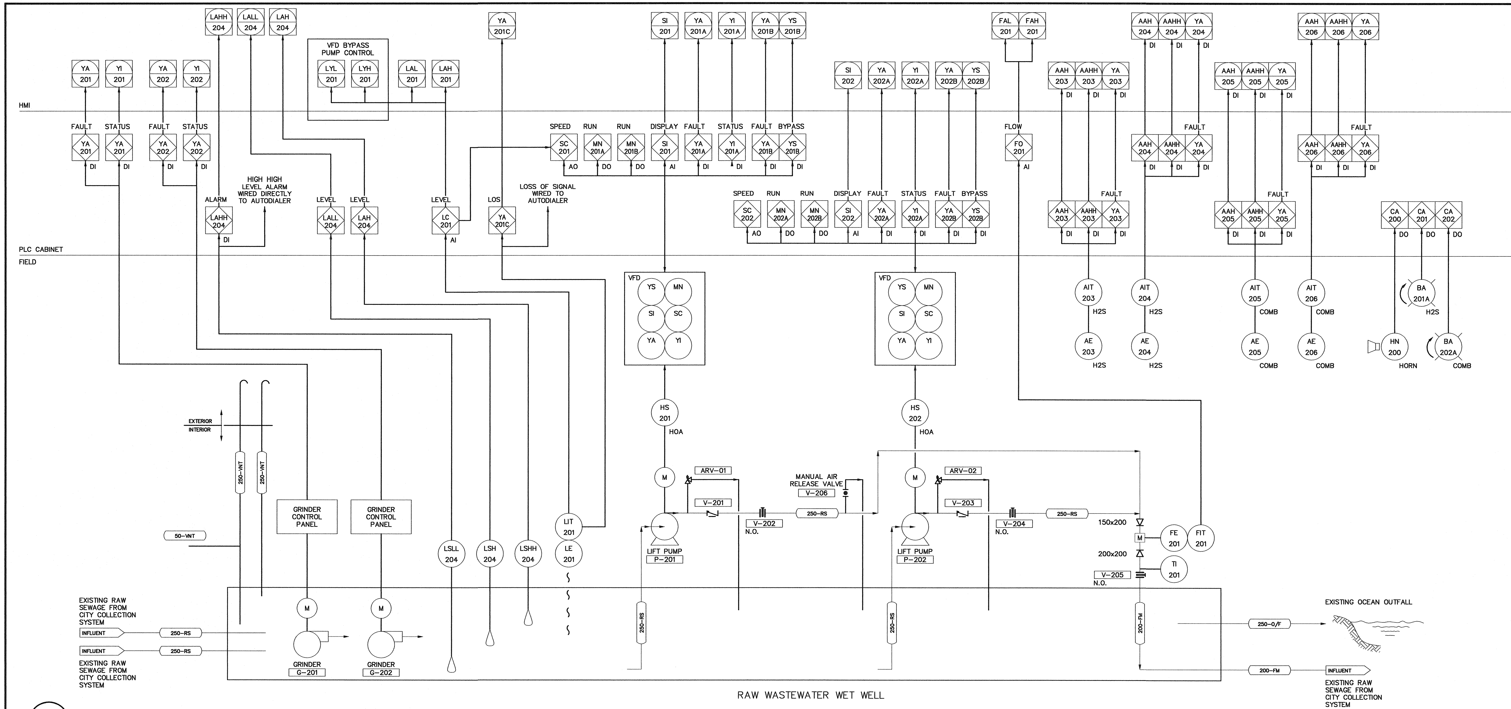
1 E5 PIPING AND INSTRUMENTATION N.T.S.
