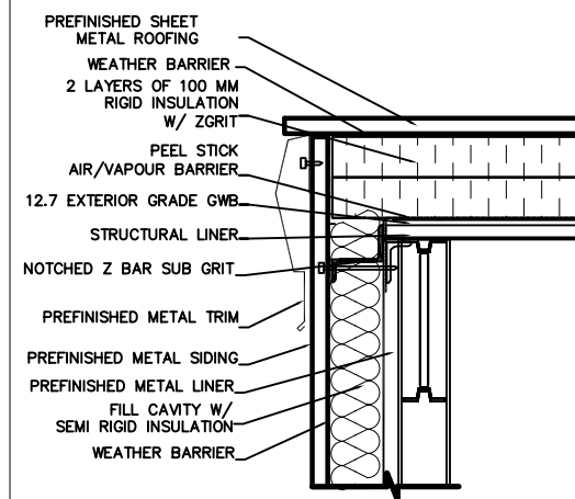
2 DETAIL #2 A151 SCALE = 1:50
