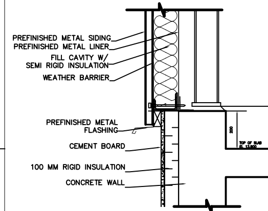
3 DETAIL #3 A151 SCALE = 1:50
