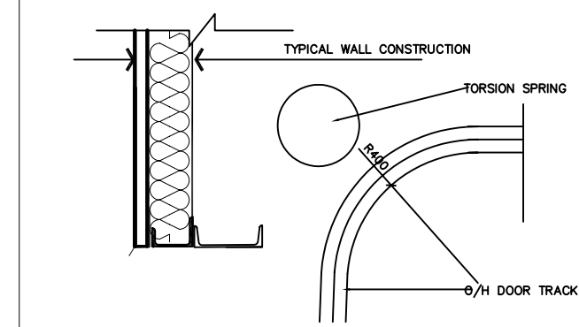
7 OVERHEAD DOOR SECTION A151 SCALE = 1:50
