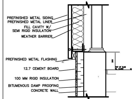
1 REMOVEABLE PANEL DETAIL #1 A151 SCALE = 1:50
