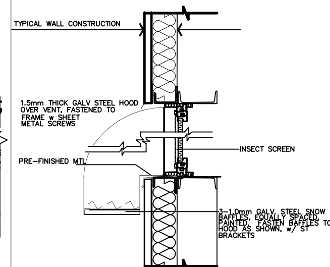
6 TYPICAL WALL PENETRATION DETAIL A151 SCALE = 1:50
