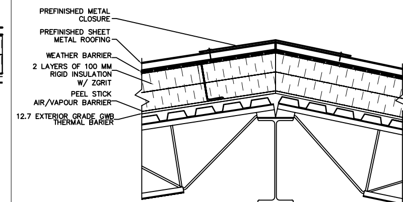
4 DETAIL #4 A151 SCALE = 1:50
