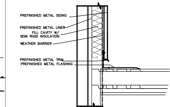
5 DETAIL #5 A151 SCALE = 1:50
