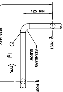
FIXED HANDRAIL CORNER
