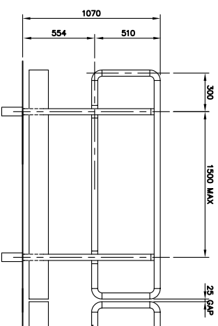
REMOVEABLE HANDRAIL ELEVATION
