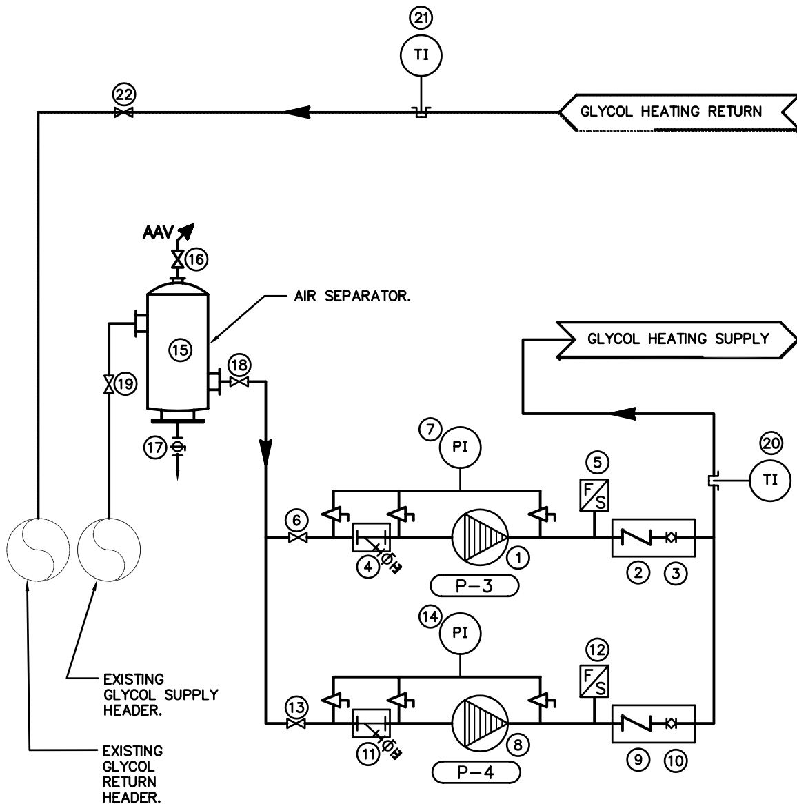
NEW HEATING PUMPS SCHEMATIC N.T.S.
