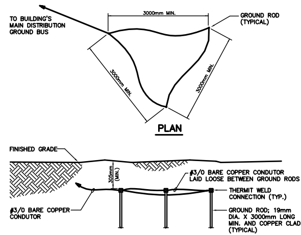
SERVICE GROUNDING DETAIL N.T.S.
