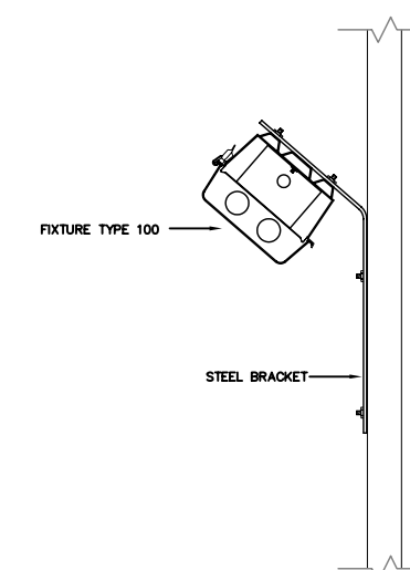
LUMINAIRE TYPE 100 - WALL MOUNTING DETAIL
