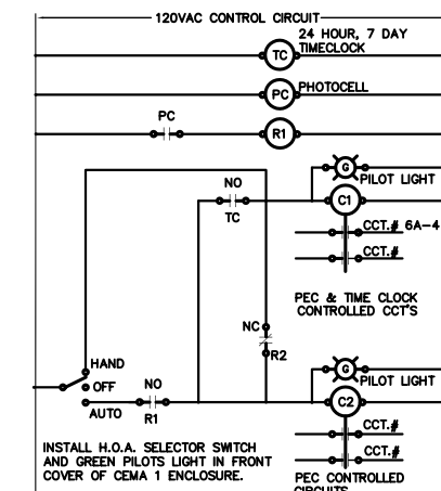
PEC EXTERIOR LIGHTING CONTROL SCHEMATIC N.T.S.
