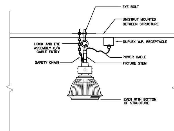
LUMINAIRE TYPE 203 & 204 - MOUNTING DETAIL N.T.S.
