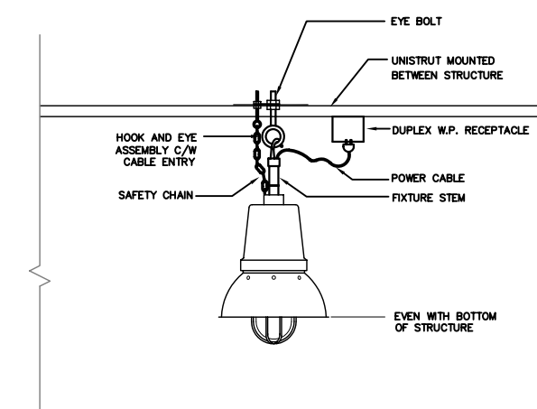
LUMINAIRE TYPE 201 – MOUNTING DETAIL N.T.S.
