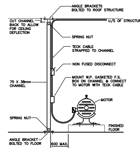
TYPICAL PROCESS MOTOR CONNECTION DETAIL N.T.S.
