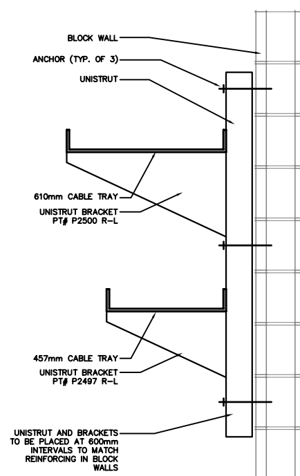
TYPICAL WALL MOUNTED TRAY DETAIL N.T.S.
