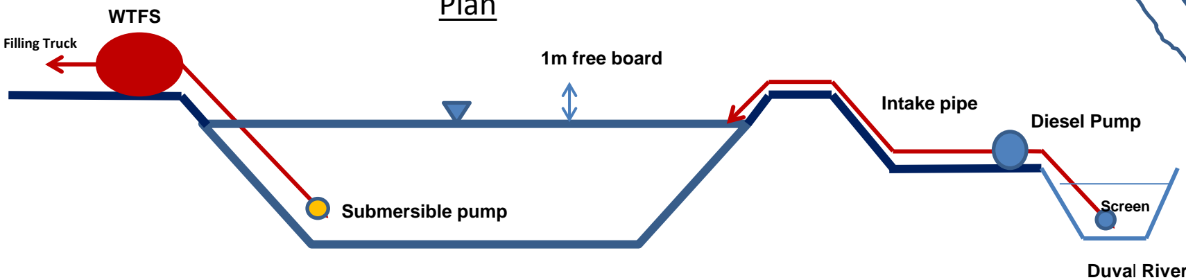
Cross Section
