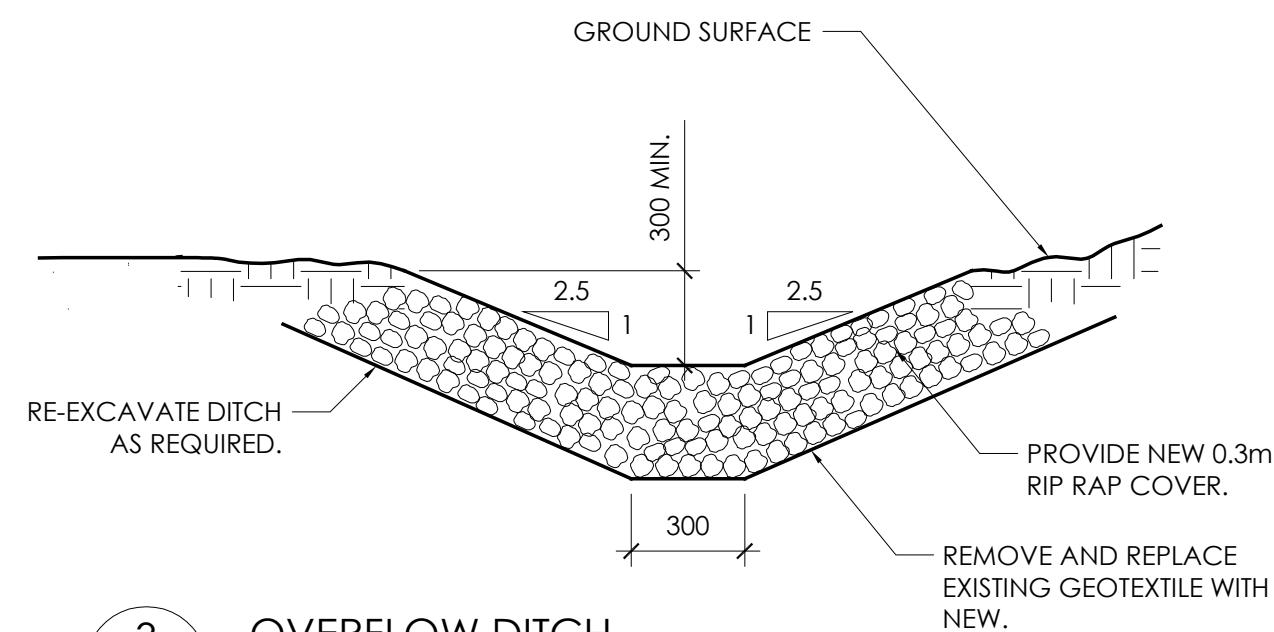
3 OVERFLOW DITCH SCALE 1:20
