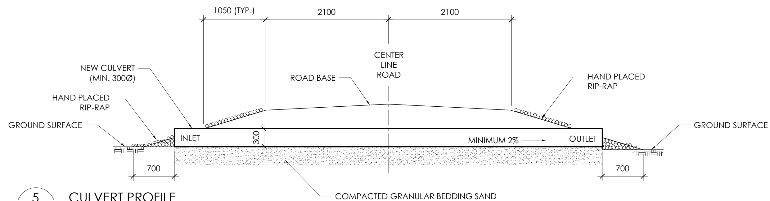
5 CULVERT PROFILE SCALE 1:40
