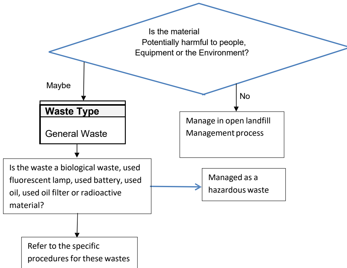
Fig. 10: Identification of Hazardous Wastes
