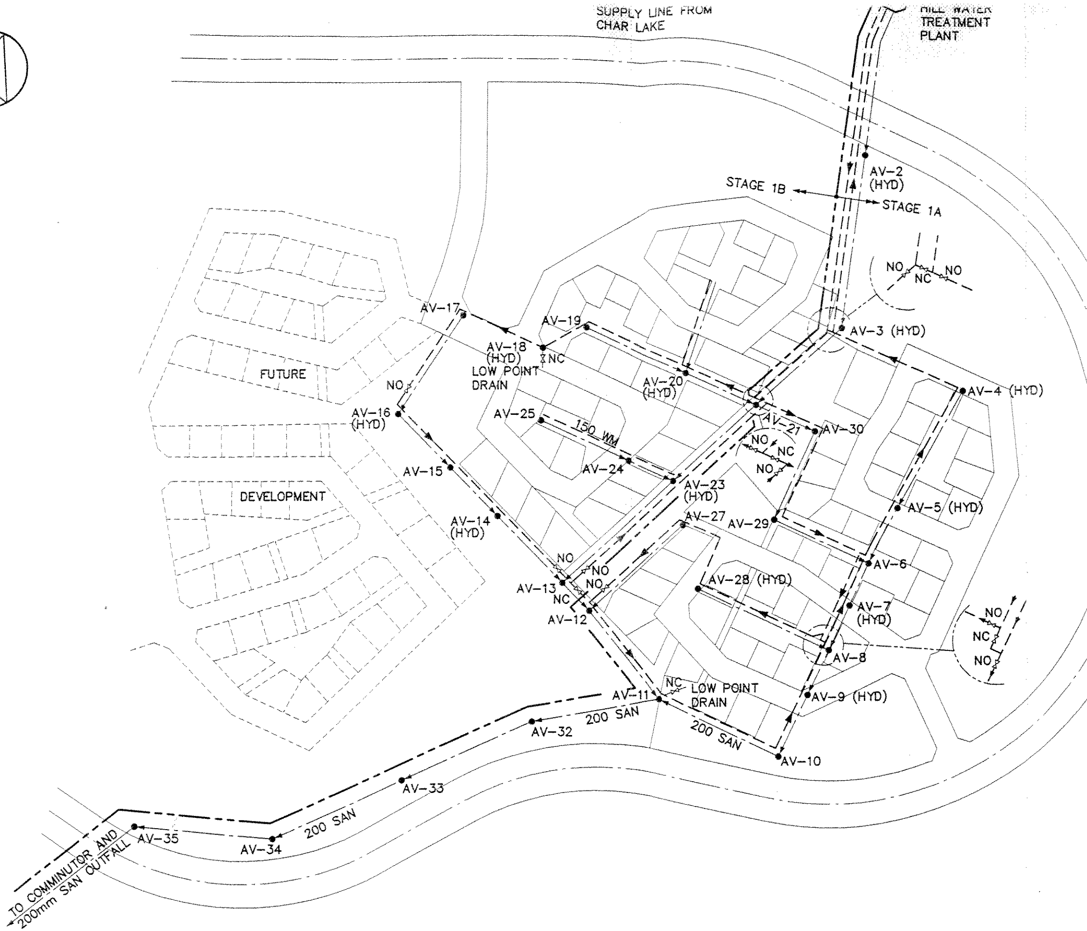
RESOLUTE BAY WATER AND SEWER EXISTING PIPING PLAN Fig. 3-2
