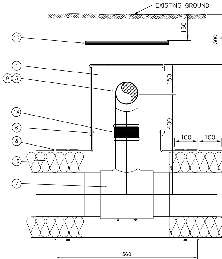
SEWER SERVICE STUB FRONT VIEW.
