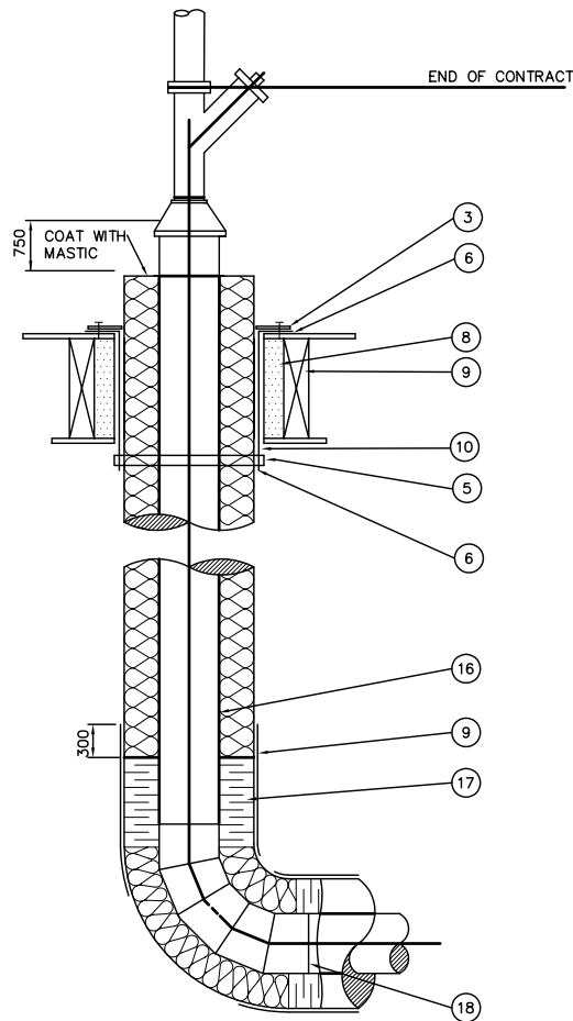
TYPICAL SANITARY SERVICE RISER N.T.S.
