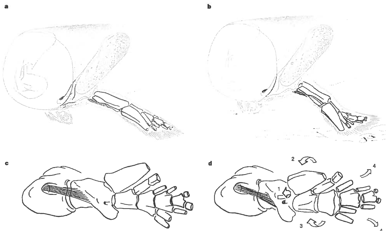
Figure 7 | Reconstruction of fin postures of Tiktaalik . a , b , Anterolateral view. c , d , Ventral view. a , c , Resting posture with the fin partially flexed at the antebrachium. In this position the radius is slightly more flexed than the ulna. b , d , Resistant contact with a firm substrate entails flexion at proximal joints and extension at distal ones. The shoulder joint is flexed by ventral
