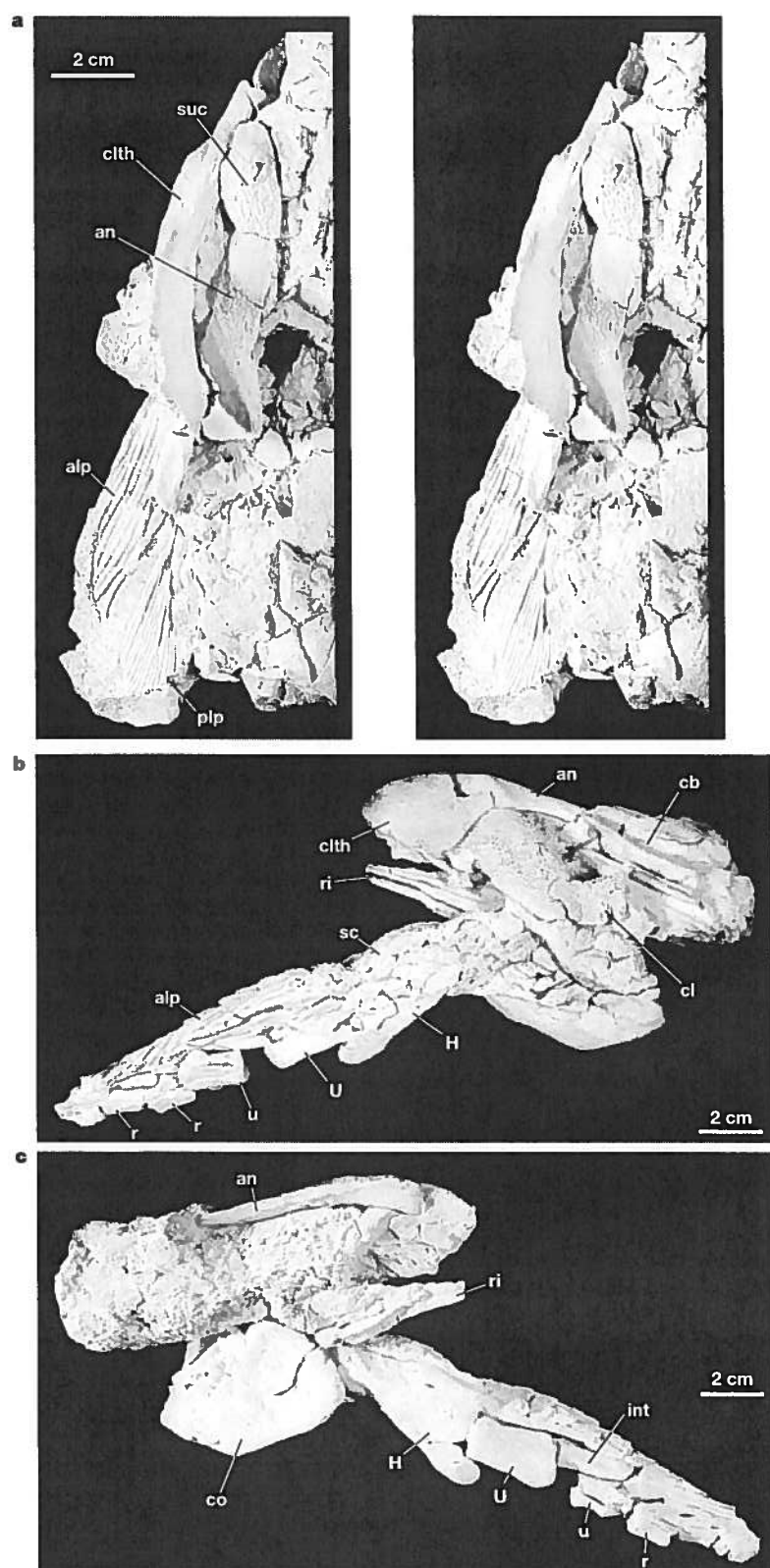
Figure 1 | Articulated pectoral fins of Tiktaalik roseae . a , Stereo pair of left pectoral fin of NUVF 108 in dorsal view showing disparity in size and position of anterior (alp) and posterior (plp) unjointed lepidotrichia and the relative position of dermal girdle elements. b , Right pectoral fin of NUVF 110 in anterior view showing preservation of anterior lepidotrichia (alp), clavicle (cl), scales (sc) and endochondral bones in articulation (H, humerus; U, ulna; u, ulnare; r, radials). The anterior lepidotrichia terminate at the elbow, thus allowing a full range of flexion at that joint. c , Right pectoral fin of NUVF 110 in ventral view showing positions of coracoid (co) and endochondral and dermal fin elements. an, anocleithrum; cb, ceratobranchial; clth, cleithrum; int, intermedium; ri, rib; suc, supracleithrum.
