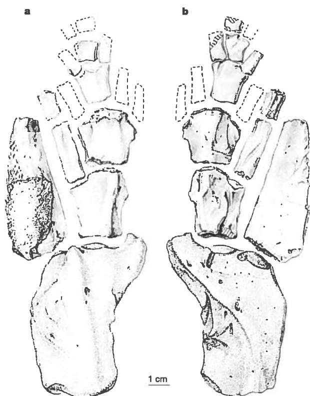
Figure 2 | Reconstruction of the right pectoral fin of Tiktaalik . a, Dorsal view; b, ventral view. Elements with stipple shading were preserved in articulation in NUFV 109 and prepared in the round. Elements with a dashed outline are reconstructed based on their presence in the articulated distal fin of NUFV 110. It is not known how many radials lie distal to the first, second and fourth in the proximal series. Note the dorsal expansion of the distal articular facets on the ulnare and third distal radial/mesomere. The dorsal expansion of these facets would have facilitated extension of the distal fin.
