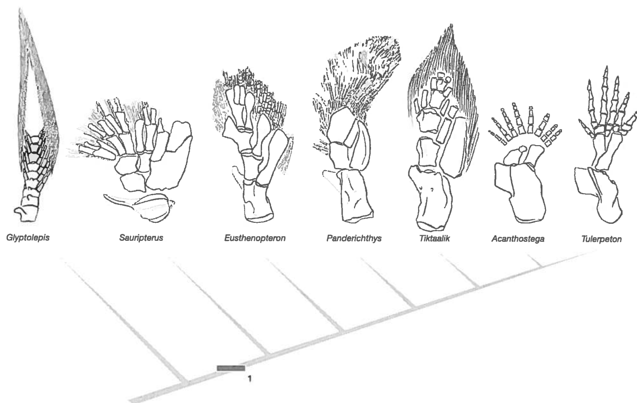
Figure 4 | Cladogram of the pectoral fins of taxa on the tetrapod stem. Unlike other tetrapodomorph fishes (1), Tiktaalik has reduced the unjointed lepidotrichia, expanded the radials to a proximal, intermediate and distal series, and established multiple transverse joints in the distal fin. The fin also retains a mosaic of features seen in basal taxa. The central axis of enlarged endochondral bones is a pattern found in basal sarcopterygians and accords with hypotheses that a primitive fin axis is homologous to autopodial bones
