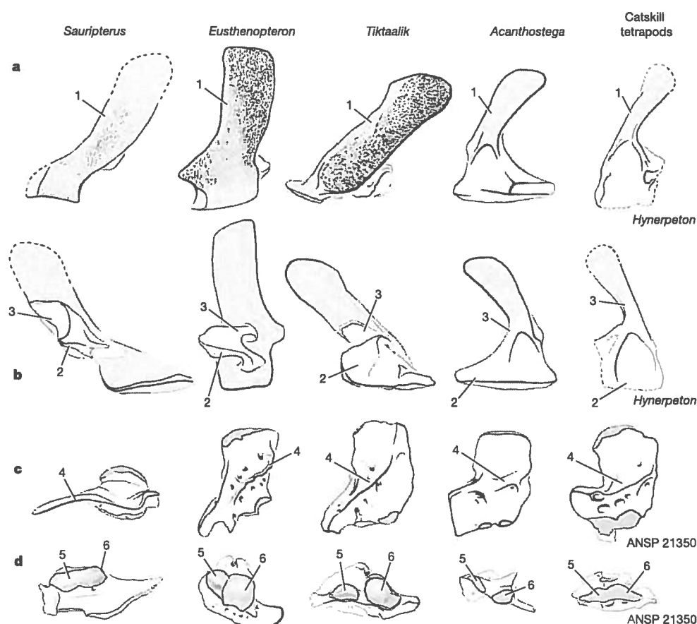
Figure 5 | A comparison of pectoral girdles and humeri in taxa along the tetrapod stem. a, b, Left pectoral girdles in lateral (a) and medial (b) views (dermal bone shaded). c, d, Left humeri in ventral view (c; articular surfaces shaded) and articular view (d; articular facets stippled; articular area shaded). Tiktaalik is intermediate between basal tetrapodomorphs and stem tetrapods in a wide range of features. a, As in basal taxa, the cleithrum (1) of Tiktaalik is heavily ornamented. Tiktaalik is intermediate in the degree to which the glenoid faces laterally, and hence, the appendage projects laterally. In both Acanthostega and Tiktaalik the appendage projects ventrolaterally from the body wall. b, Tiktaalik has an enlarged scapulocoracoid relative to
