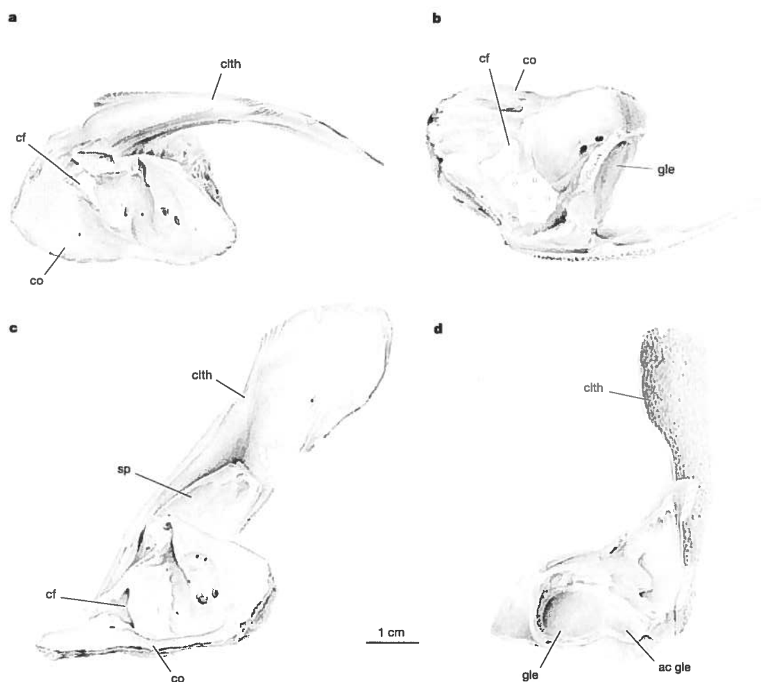
Figure 3 | Isolated right shoulder girdle of Tiktaalik (NUFV 112). a , Dorsal view; b , ventral view; c , medial view; d , posterior view. ac gle, anterior cam of glenoid facet; cf, coracoid foramen; clth, cleithrum; co, coracoid; gle, glenoid facet; sp, scapular process. The hatched area is covered by matrix.
