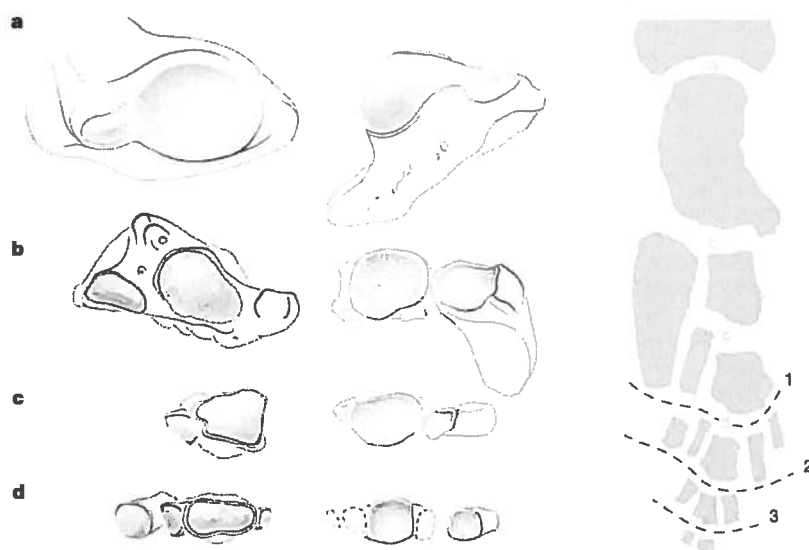
Figure 6 | Apposing joint surfaces of the left pectoral fin of NUV 109 in articular view. a , The shoulder joint consists of a large, shallow ball and socket posteriorly and a small accessory cam anteriorly. The cam serves to limit humeral protraction and supination. b , At the elbow joint, both epipodial facets of the humerus face slightly ventrally, with the radial facet offset anterioventrally from that for the ulna. c , The joints of the ulna and intermedium with the ulna are also offset from one another. As in the
