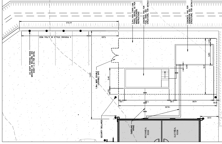
ENCLOSURE PLAN 1:100 SCALE 1:100 METERS
