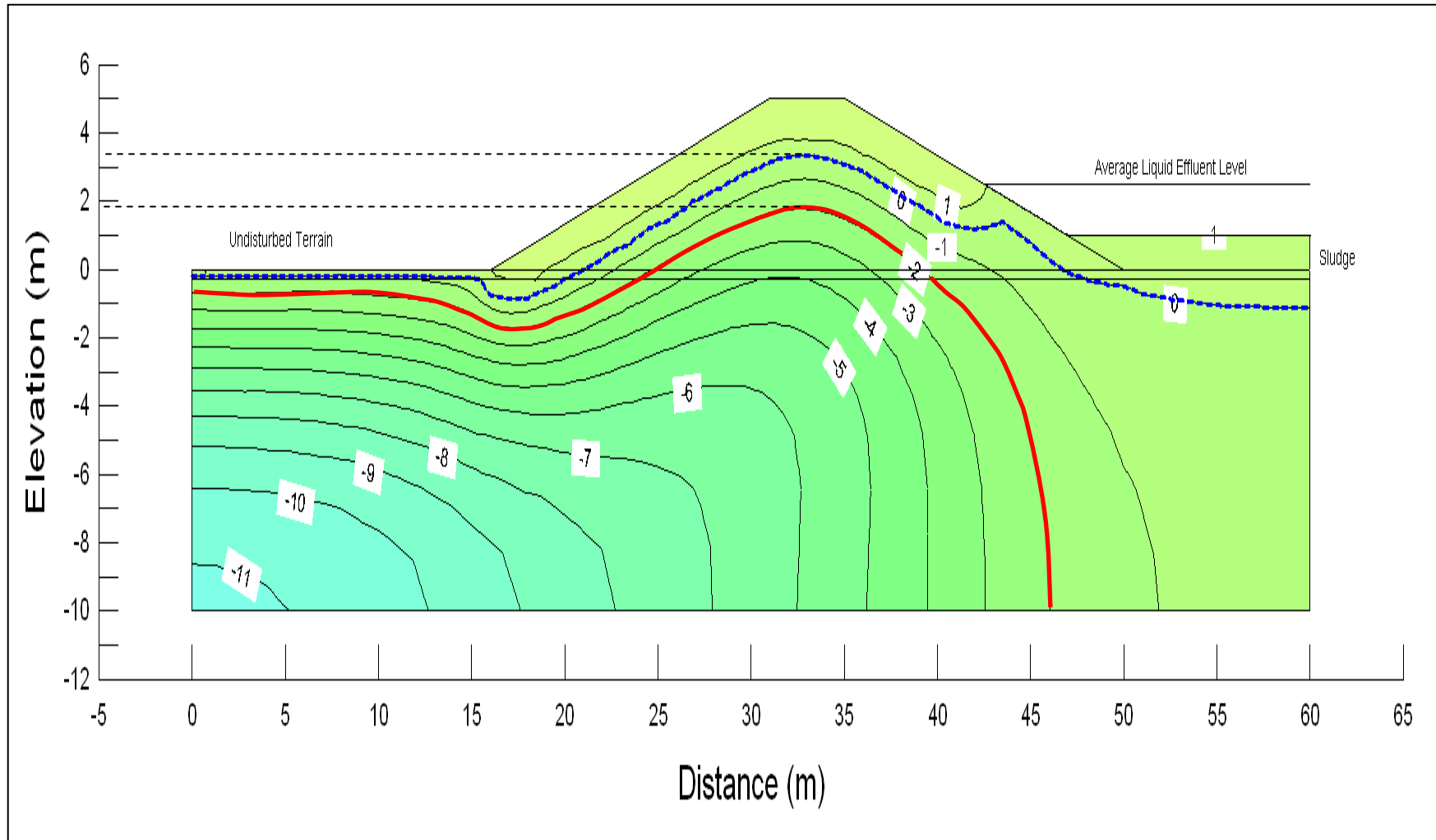
Figure 4-1. Cross-section of dyke structure showing ground temperature contours at maximum thaw during years 1 through 5. Temperature contours for years 5 through 20 would be the same. No climate warming effects are included.
