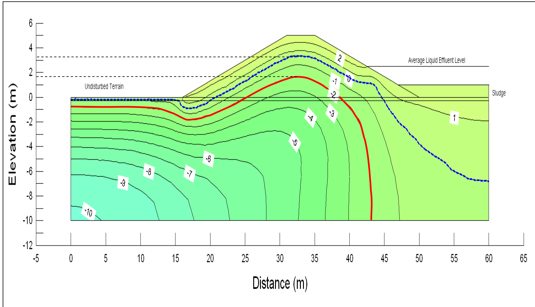
Figure 4-2. Cross-section of dyke structure showing ground temperature contours at maximum thaw after 20 years. Climate warming effects are included.
