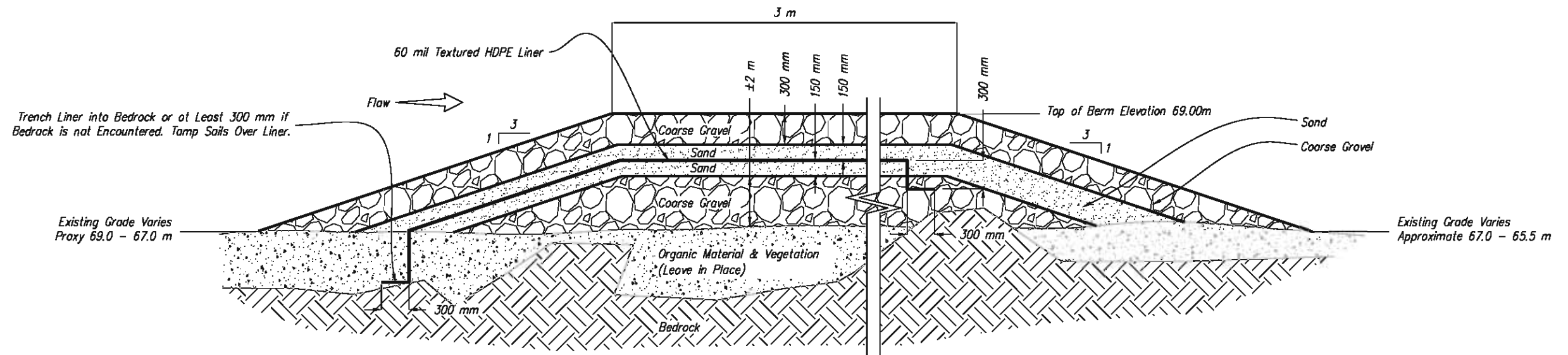
Holding Cell Berm Cross Section - A Scale: None
