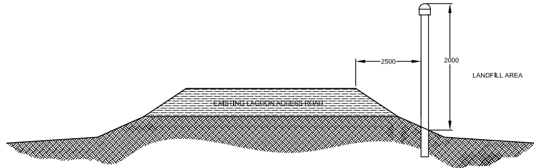
6 SECTION 4: FENCE ON THE SHOULDER OF EXISTING ROAD NOT TO SCALE DIMENSIONS IN mm
