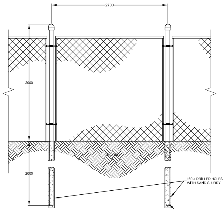
FENCE DETAIL DIMENSIONS IN mm
