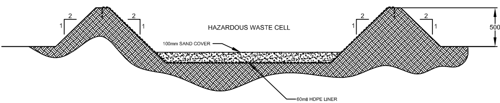
5 SAND BASE DIMENSIONS IN mm
