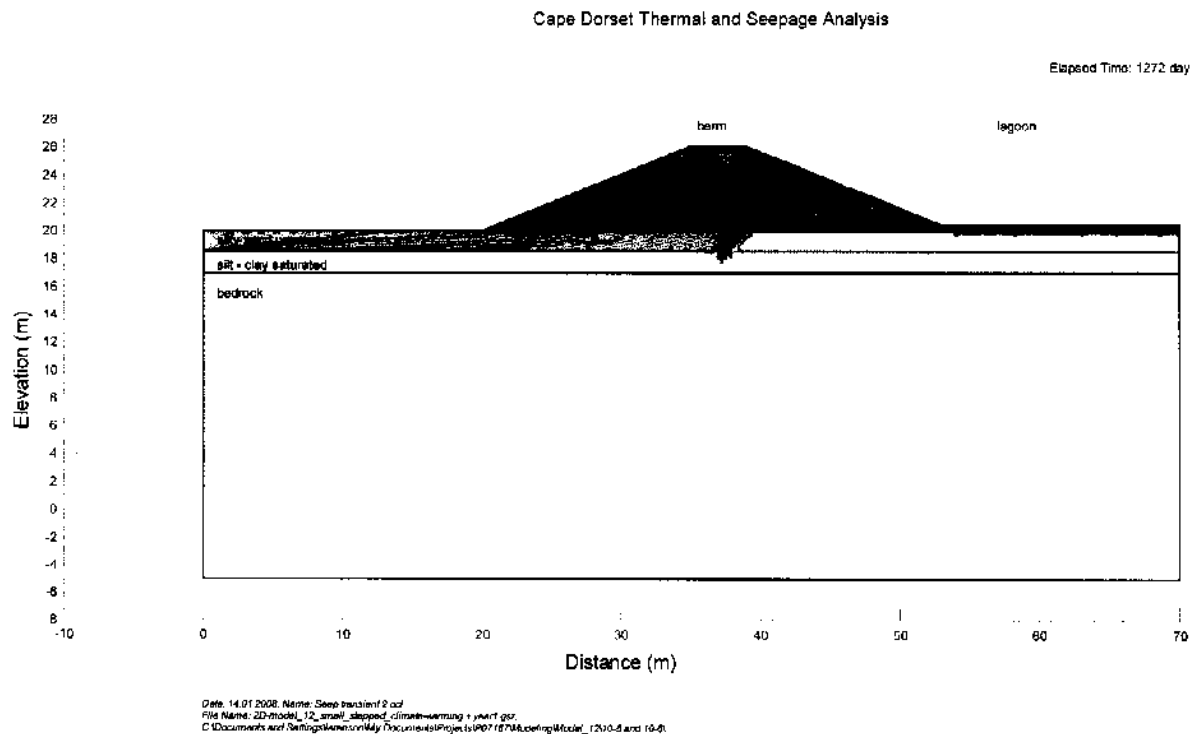
Figure 25. Predicted piezometric surfaces during year 2 of operation.
