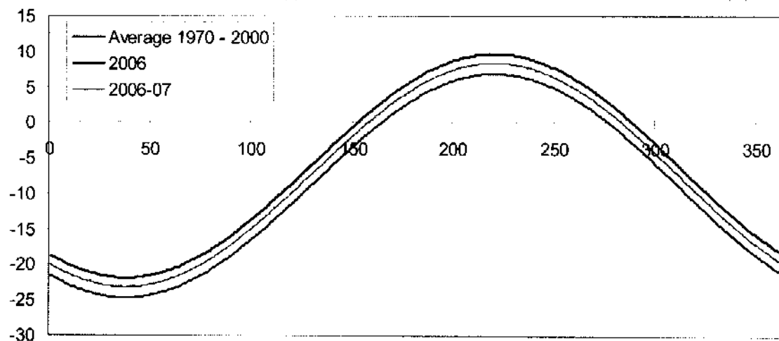
Figure 2. Sinusoidal air temperature variations used in geothermal analysis. Day 0 refers to January 1.
