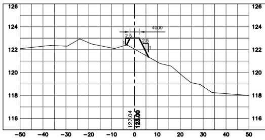
7 EAST BERM SECTION 0+010(2) 109/109 SCALE 1:750h 1:150v
