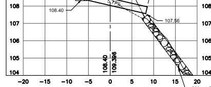
17 CULVERT SECTION AT 0+725.35 109/109 SCALE 1:400h 1:100v
