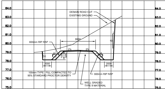
1 TYPICAL ROAD SECTION (CUT)(2) 109/109 SCALE 1:200h 1:100v
