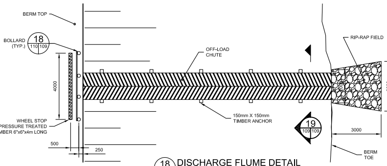
18 DISCHARGE FLUME DETAIL 109/109 SCALE 1:100
