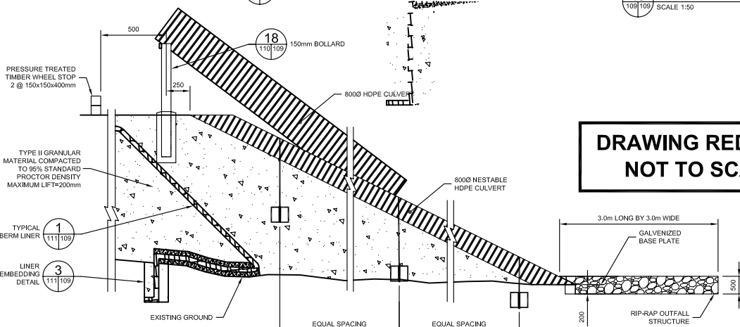
20 DISCHARGE FLUME SECTION 109/109 SCALE NTS
