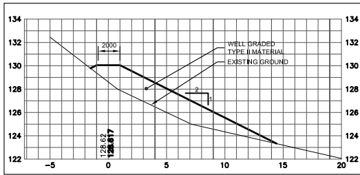
5 NORTH BERM SECTION 0+025(2) 109/109 SCALE 1:200h 1:200v
