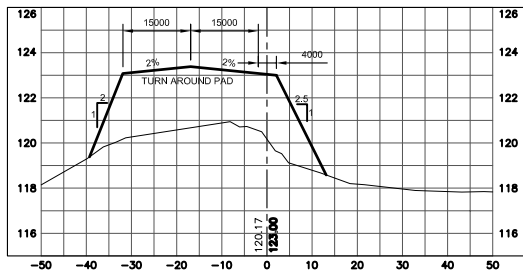
8 EAST BERM SECTION 0+050(2) 109/109 SCALE 1:750h 1:150v
