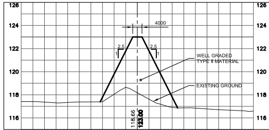
6 WEST BERM SECTION 0+140(2) 109/109 SCALE 1:750h 1:150v
