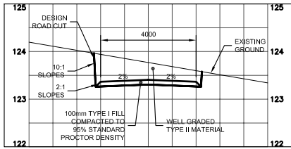
3 LAGOON ROAD SECTION (CUT)(2) 109/109 SCALE 1:100h 1:50v
