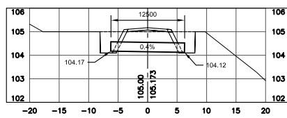
15 CULVERT SECTION AT 0+595 109/109 SCALE 1:400h 1:100v
