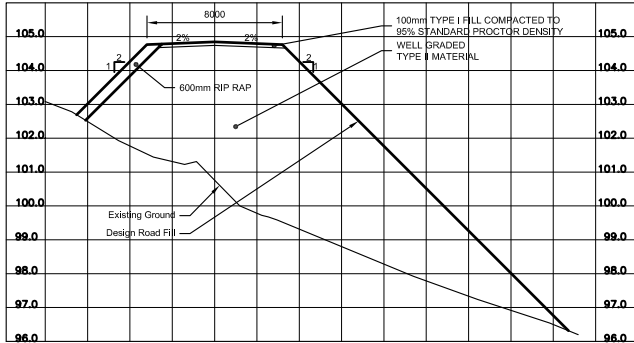
2 TYPICAL ROAD SECTION (FILL) 109/109 SCALE 1:200h 1:100v
