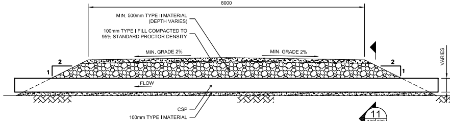
10 TYPICAL CULVERT DETAIL 109/109 SCALE 1:50
