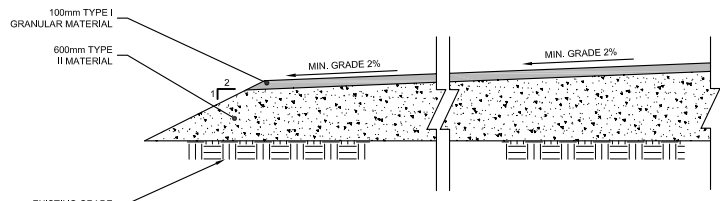
9 TRUCK TURNAROUND PAD SECTION 109/109 SCALE 1:40
