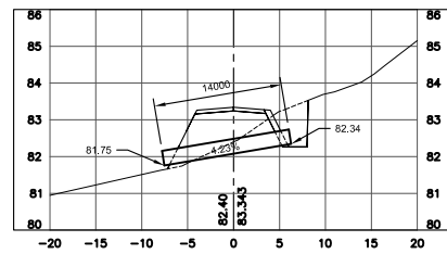
13 CULVERT SECTION AT 0+210.41 109/109 SCALE 1:400h 1:100v
