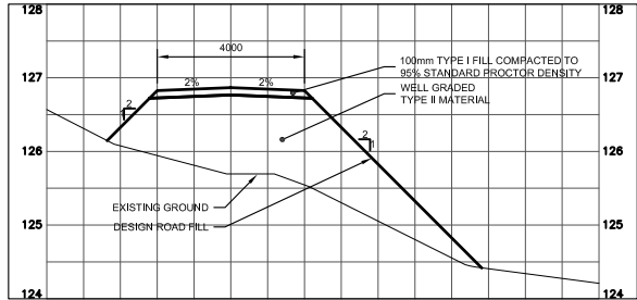
4 LAGOON ROAD SECTION (FILL)(2) 109/109 SCALE 1:100h 1:50v
