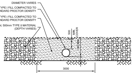
11 CULVERT SECTION 109/109 SCALE 1:50
