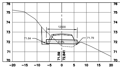
12 CULVERT SECTION AT 0+019.70 109/109 SCALE 1:400h 1:100v
