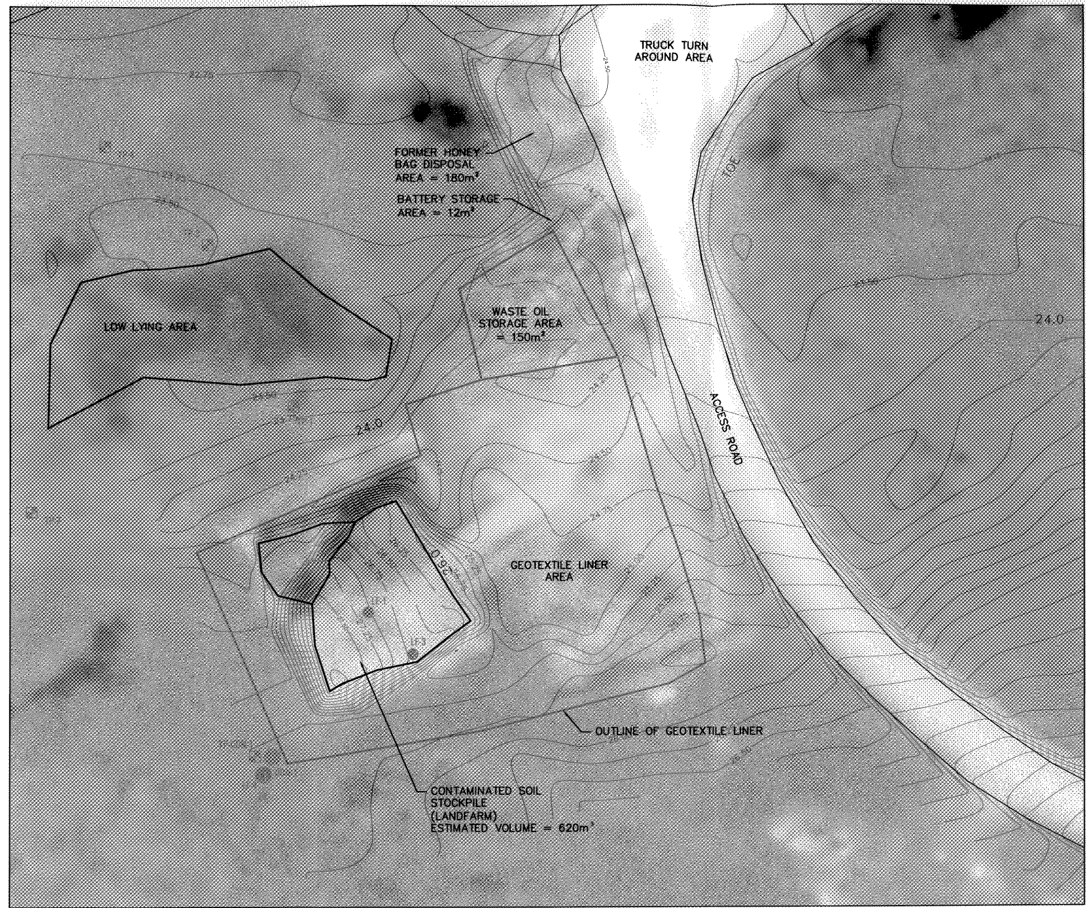
FIGURE 7 HAMLET OF KUGLUKTUK SEWAGE TREATMENT FACILITY & SOLID WASTE MANAGEMENT FACILITY DETAILED DESIGN - MARCH 2007 CONTAMINATED SOIL AND WASTE OIL STORAGE AREA
