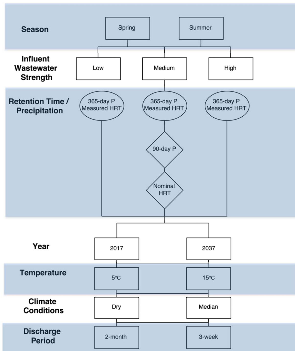
Figure 4. Flow chart of the factors and scenarios assessed within treatment performance modeling.
