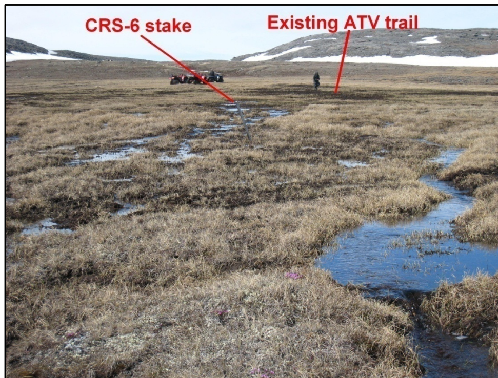
Photo 22 CRS-6 crossing stake located at Km 6.2 of the proposed access road route, note lack of defined channel at crossing and existing ATV trail in background; north aspect.
