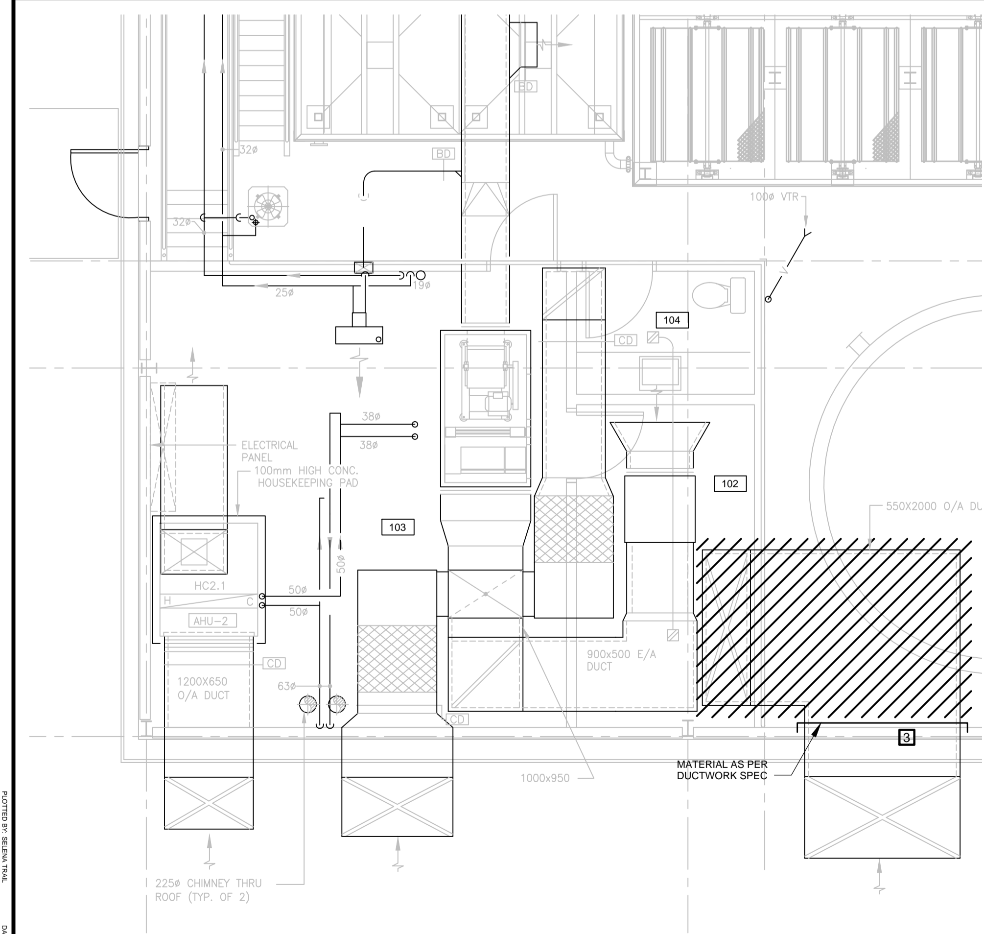
PARTIAL FLOOR PLAN - UPPER LEVEL
