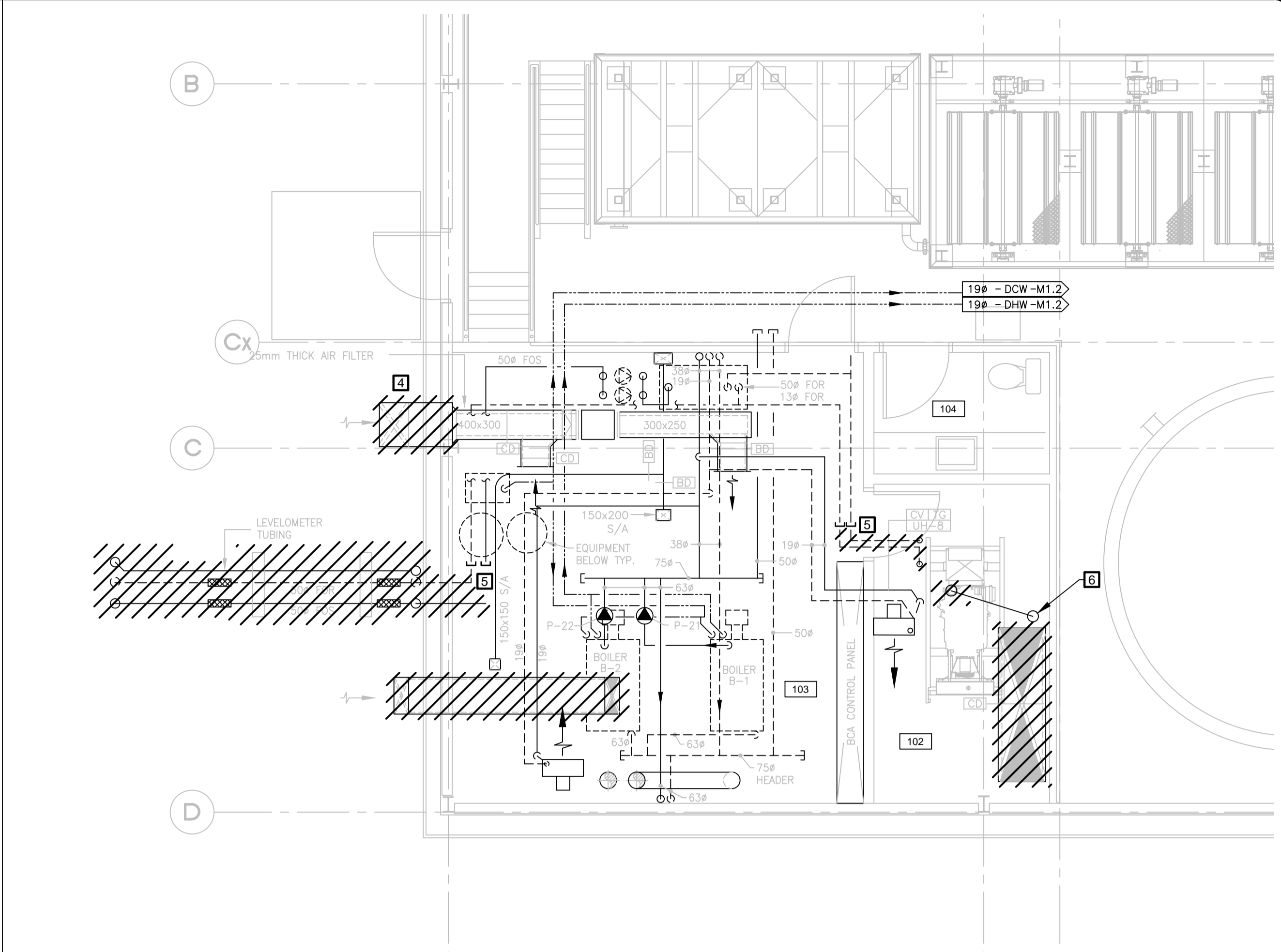
PARTIAL FLOOR PLAN - MECHANICAL ROOM - HIGH LEVEL
