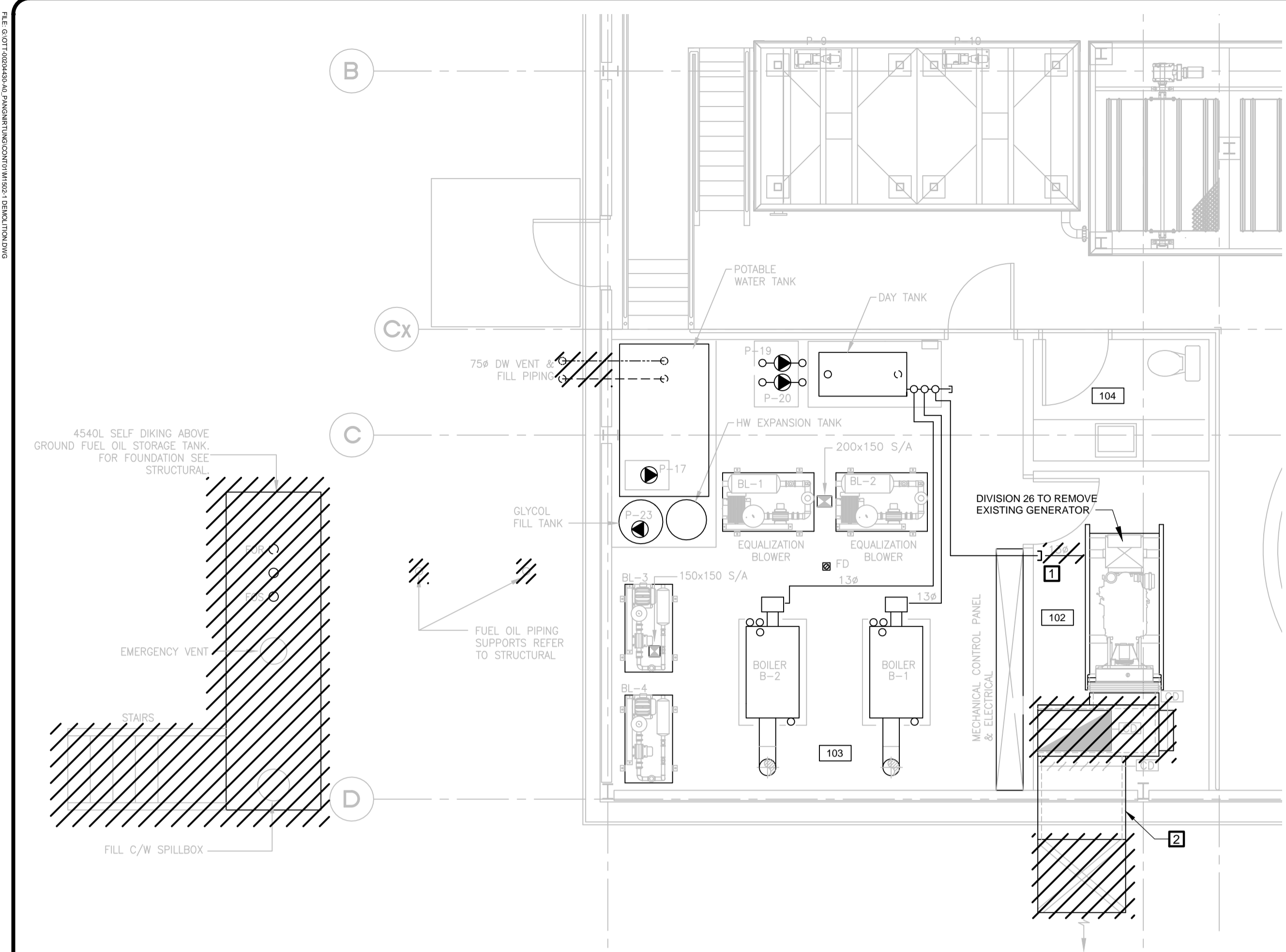
PARTIAL FLOOR PLAN - MECHANICAL ROOM - LOW LEVEL
