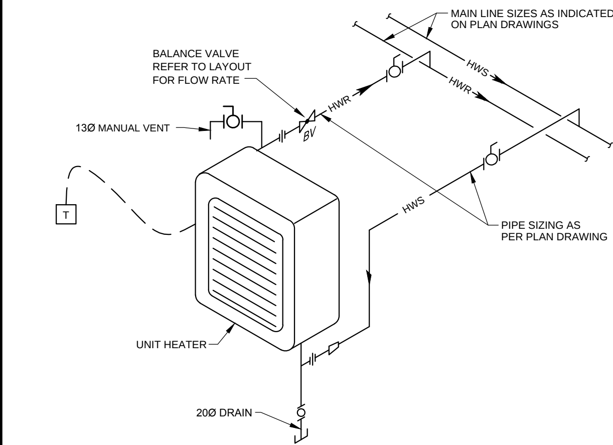
DETAIL TYPICAL HORIZONTAL UNIT HEATER PIPING
