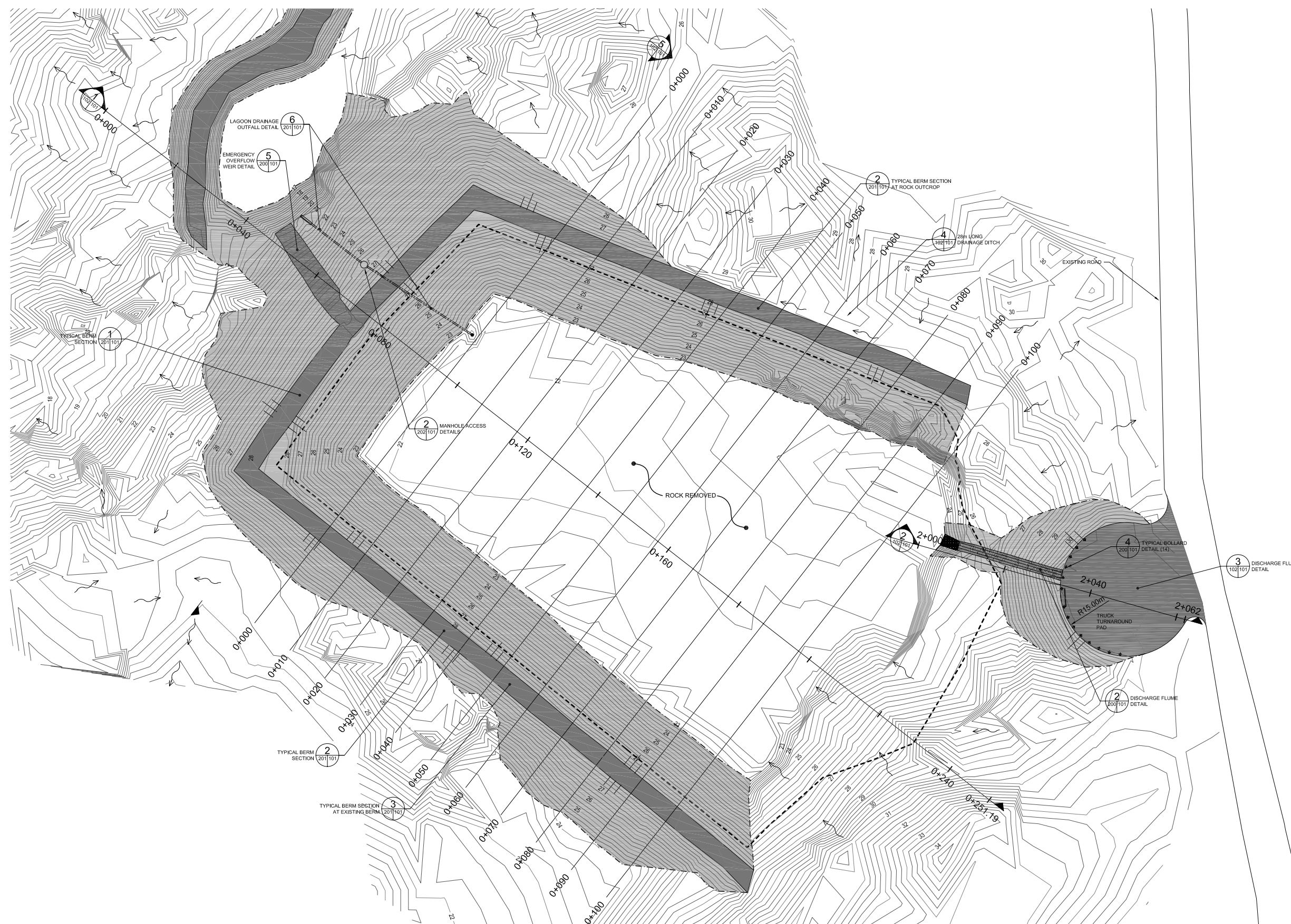
1 LAGOON DESIGN SCALE 1:500
