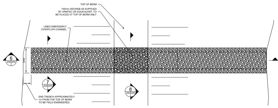
5 EMERGENCY OVERFLOW WEIR DETAIL SCALE 1:100
