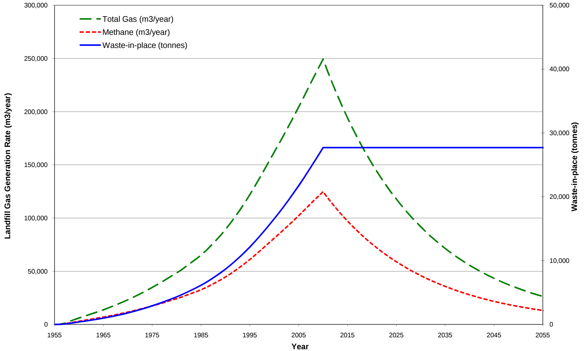
Figure 5 - Rankin Inlet Waste and Landfill Gas Generation with Time
