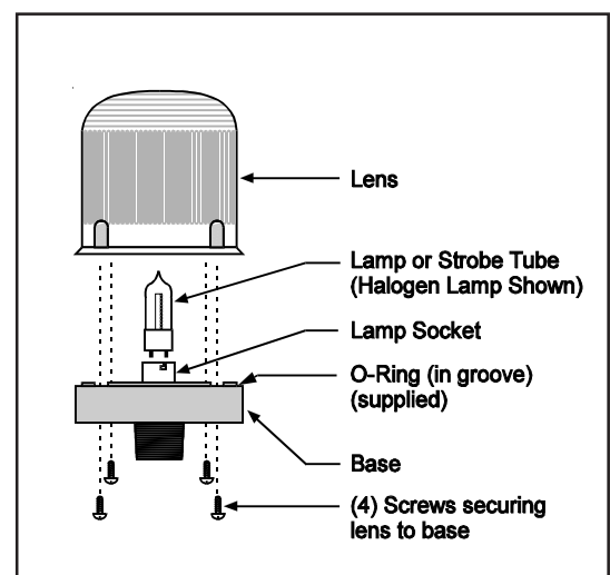
Figure 3. Lamp Replacement
