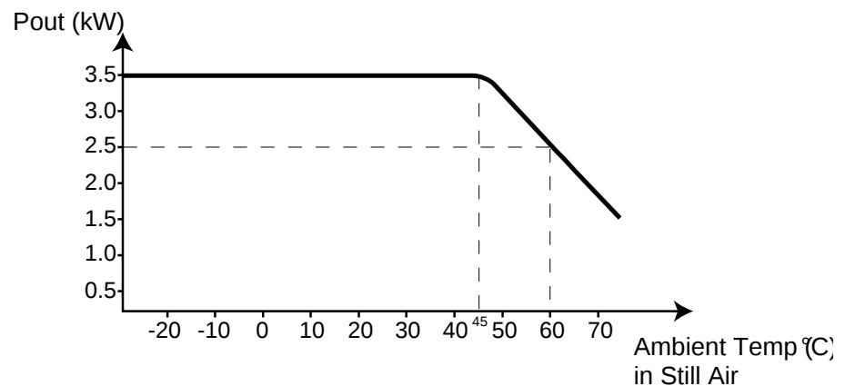
Figure A-1 Output Power vs. Ambient Temperature
