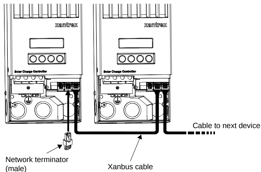
Figure 2-17 Daisy Chain Layout
