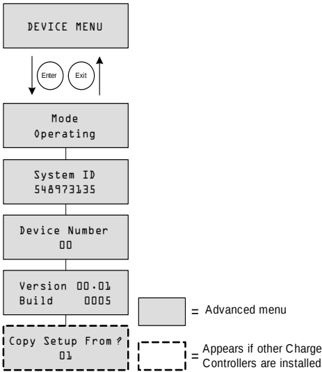
Figure 3-7 Device Menu
