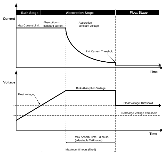
Figure 1-4 Three-stage Battery Charging Cycle a
