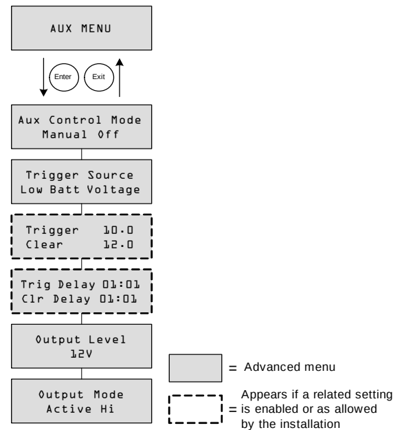
Figure 3-5 Aux Menu
