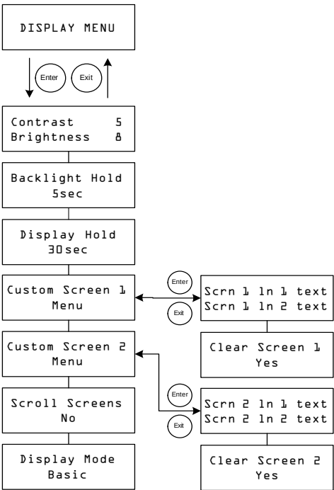
Figure 3-6 Display Menu
