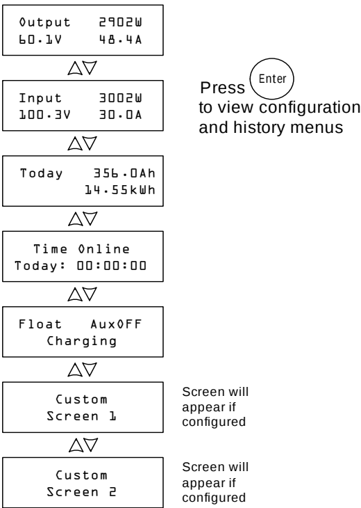
Figure 4-1 Operating Screens
