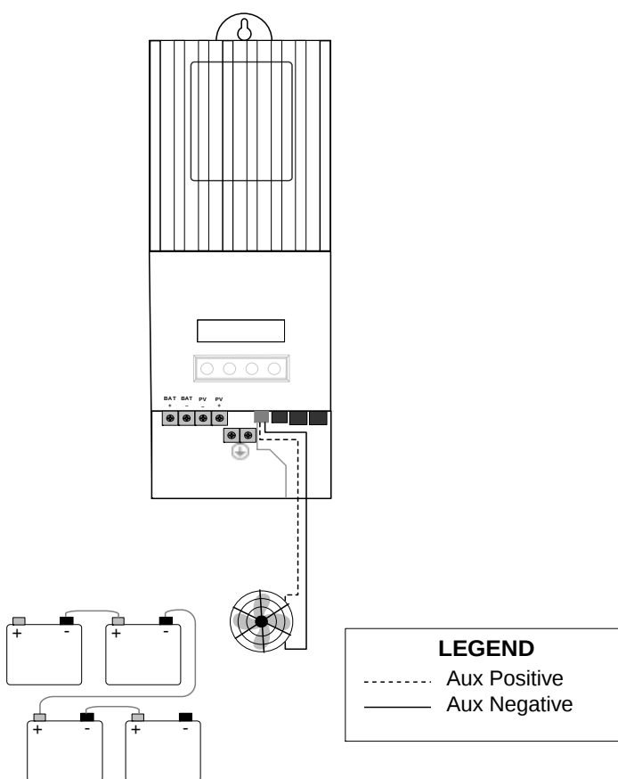
Figure 2-11 Auxiliary Output Vent Fan Application
