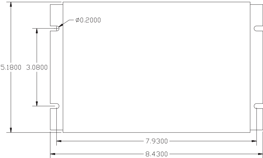
Figure 9 Mounting Detail
