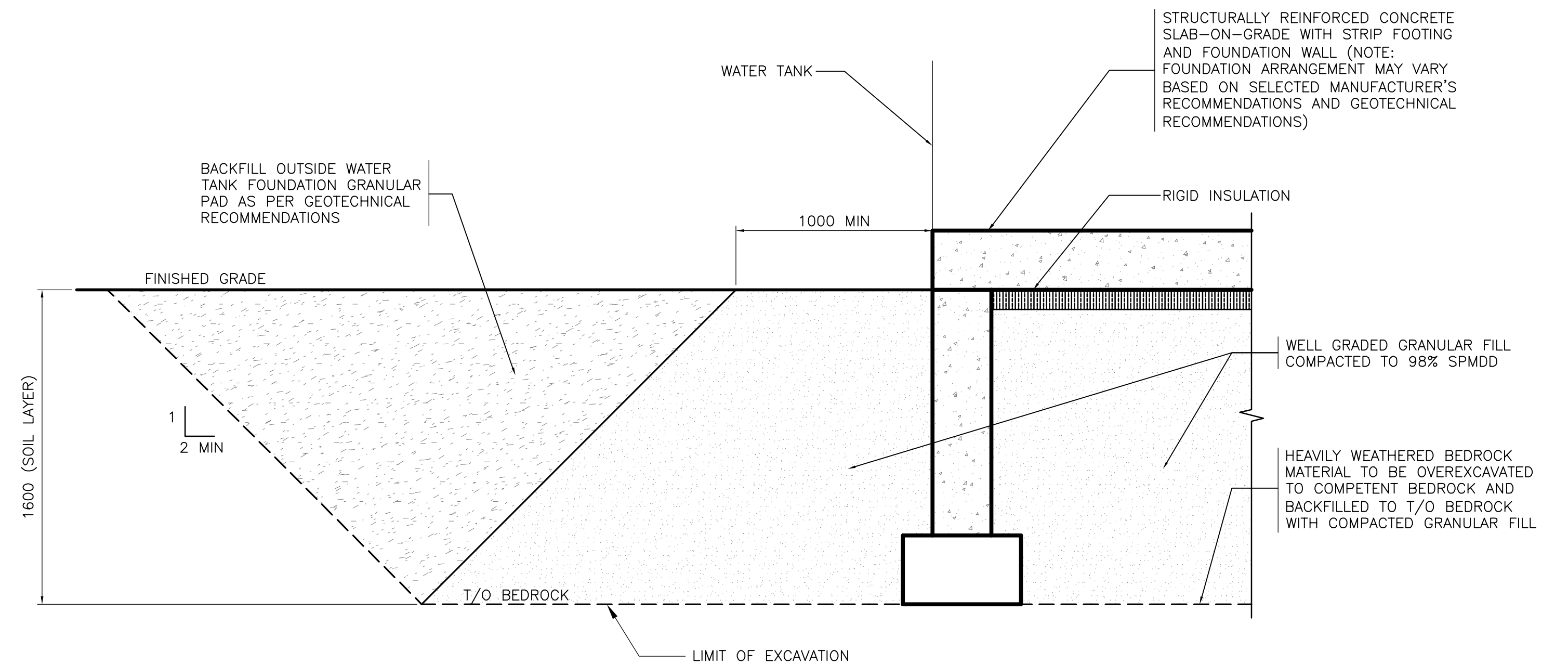
C TYPICAL TANK FOUNDATION SECTION 1:20
