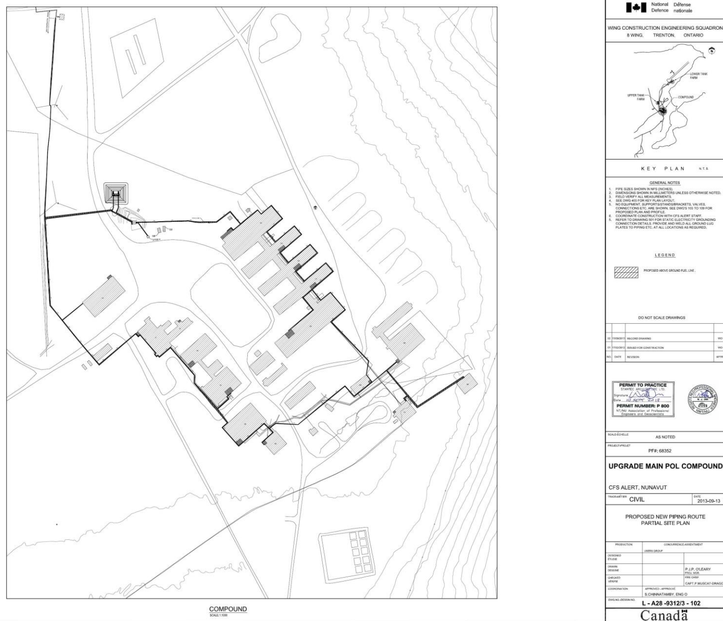
Figure 3. New aboveground POL pipeline at CFS Alert (Sept 2013).
