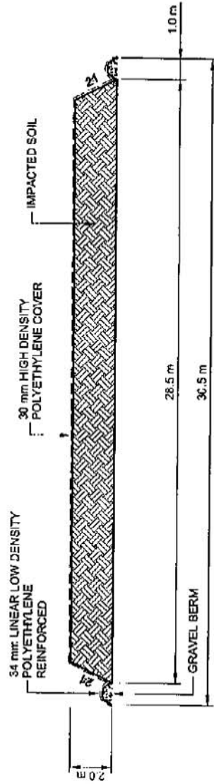
SECTION B-B
