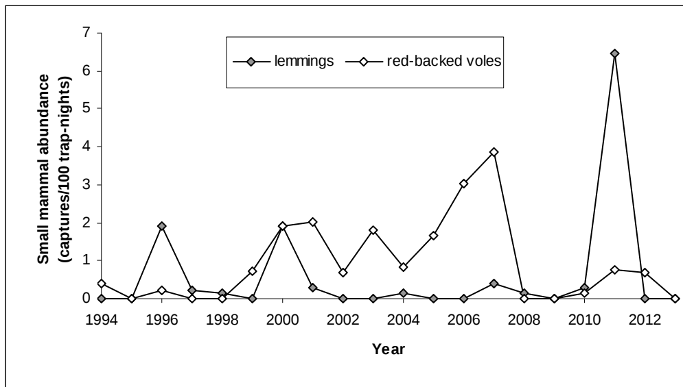
Figure 1. Small mammal abundance at Karrak Lake in 1994 to 2013.
