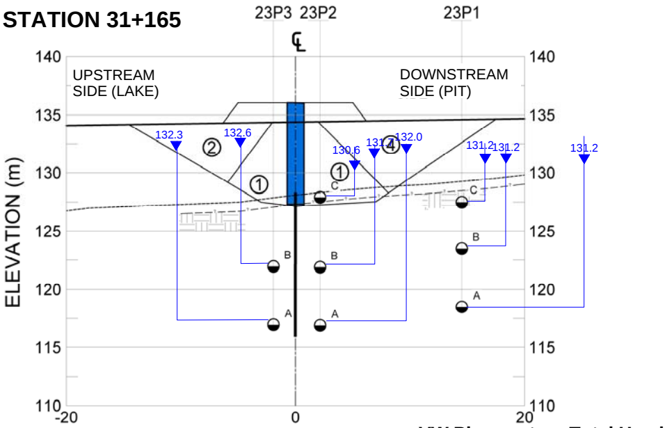
VW Piezometer - Total Head
