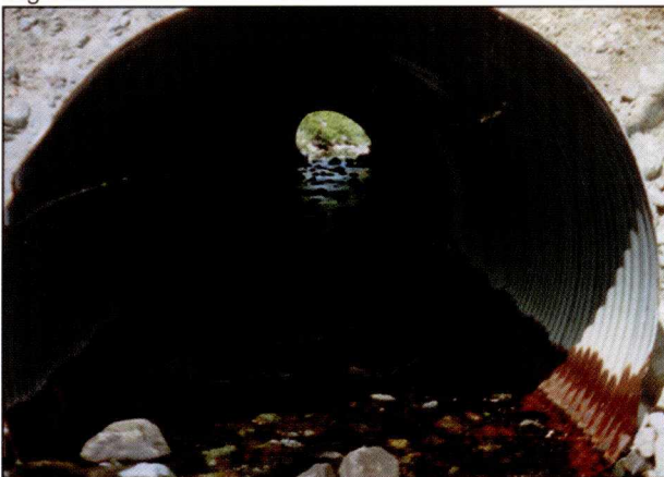
Figure 3. Countersunk Culvert
