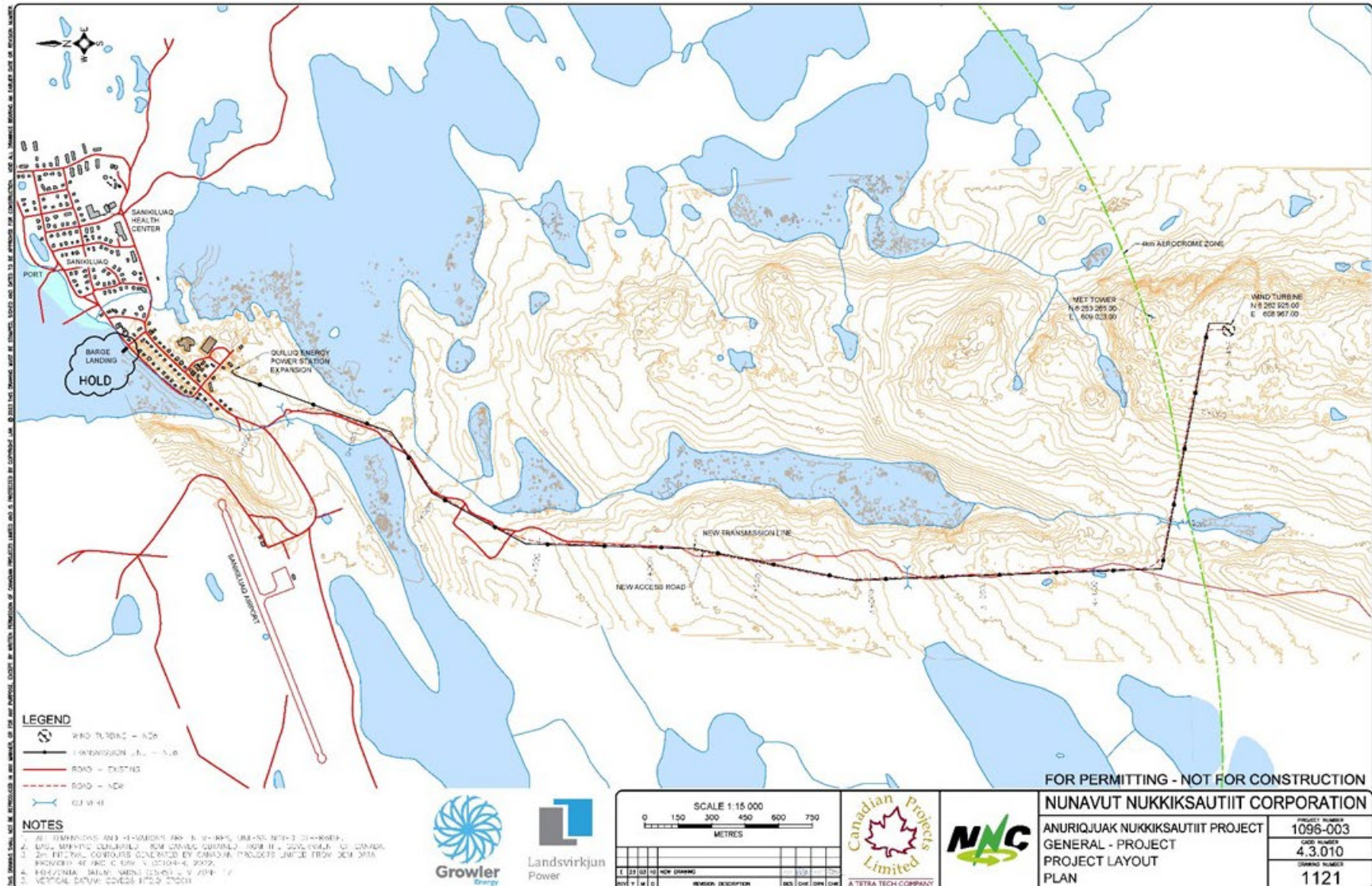
Figure 2.1 Project Layout.
