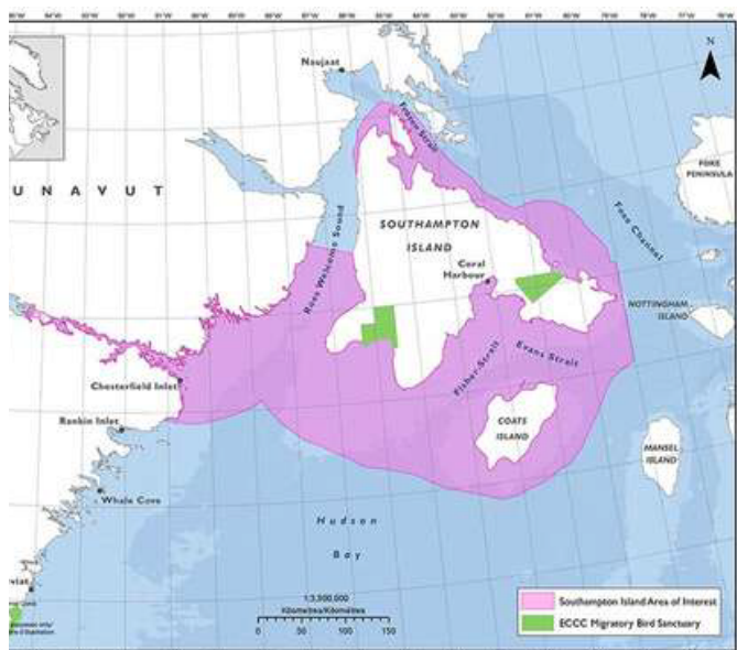
\exists^b \rho \in \Delta L^\gamma \Gamma^b \quad \Gamma \triangleleft \sigma^\gamma \rho \sigma^\gamma b^\gamma \Delta \triangleright \varphi L \varphi \Gamma^c.
