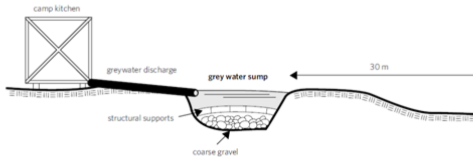
FIGURE 22. A properly excavated greywater sump.
