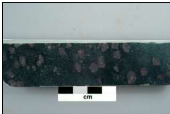
Photograph of 16729. Note the garnet porphyroblasts.
