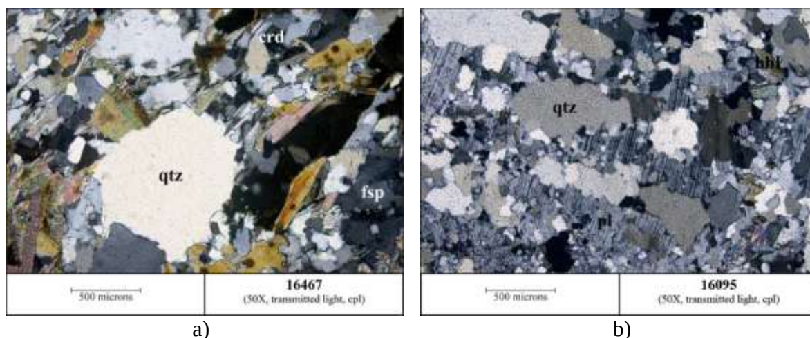
Figure 1. Photomicrographs illustrating the occurrence of quartz and feldspar. a) Photomicrograph of relatively coarse quartz grains in a matrix of granoblastic quartz and cordierite with decussate biotite. b) Photomicrographs of plagioclase porphyroblasts in a matrix of granoblastic quartz and feldspar with disseminated hornblende.
